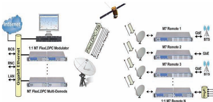
POINT-TO-MULTIPOINT EXAMPLE
